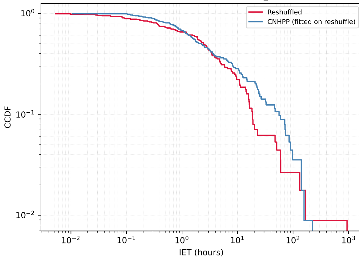
User 459294324 - Reshuffled vs CNHPP A_{\text{fit}}=0.7819
